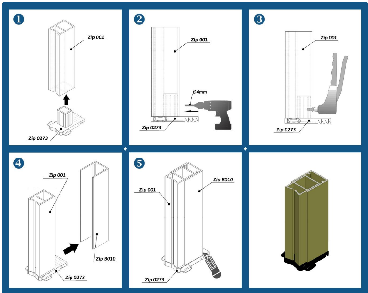
Zip 0273 - Track Bottom Cap is only required when the bottom of the track does not meet a surface.
